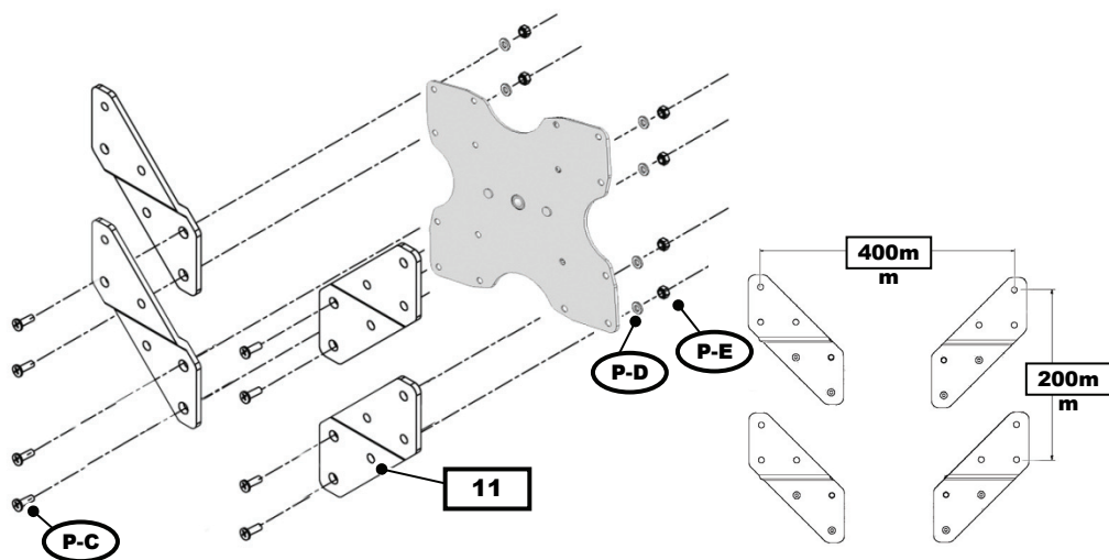
VESA – 400mm x 400mm, 300mm x 300mm
