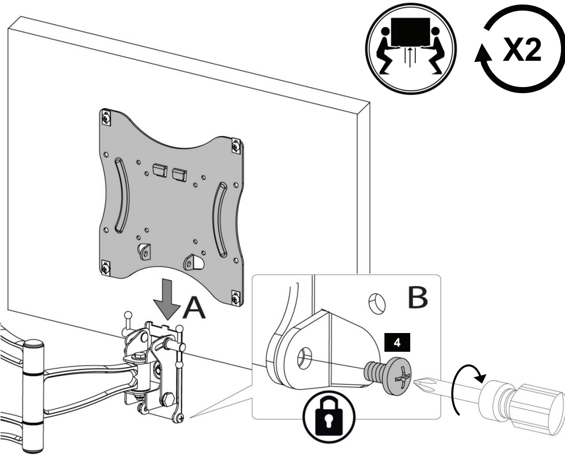
Adapters (Part#3) not shown for clarity
