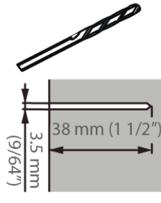
Wood Stud Pilot Hole BIT NOT INCLUDED
