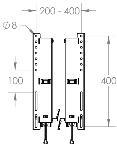
PANEL ATTACHMENT - VESA COMPATABILITY (mm)
