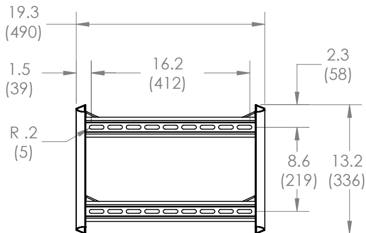
WALL MOUNTING
