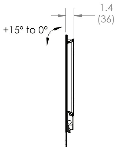
MOUNTING PROFILE
